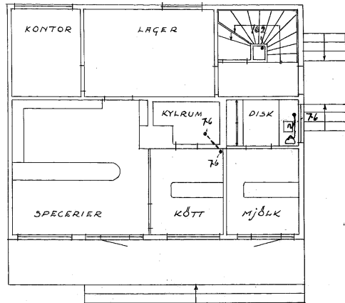
BOTTENPLAN
