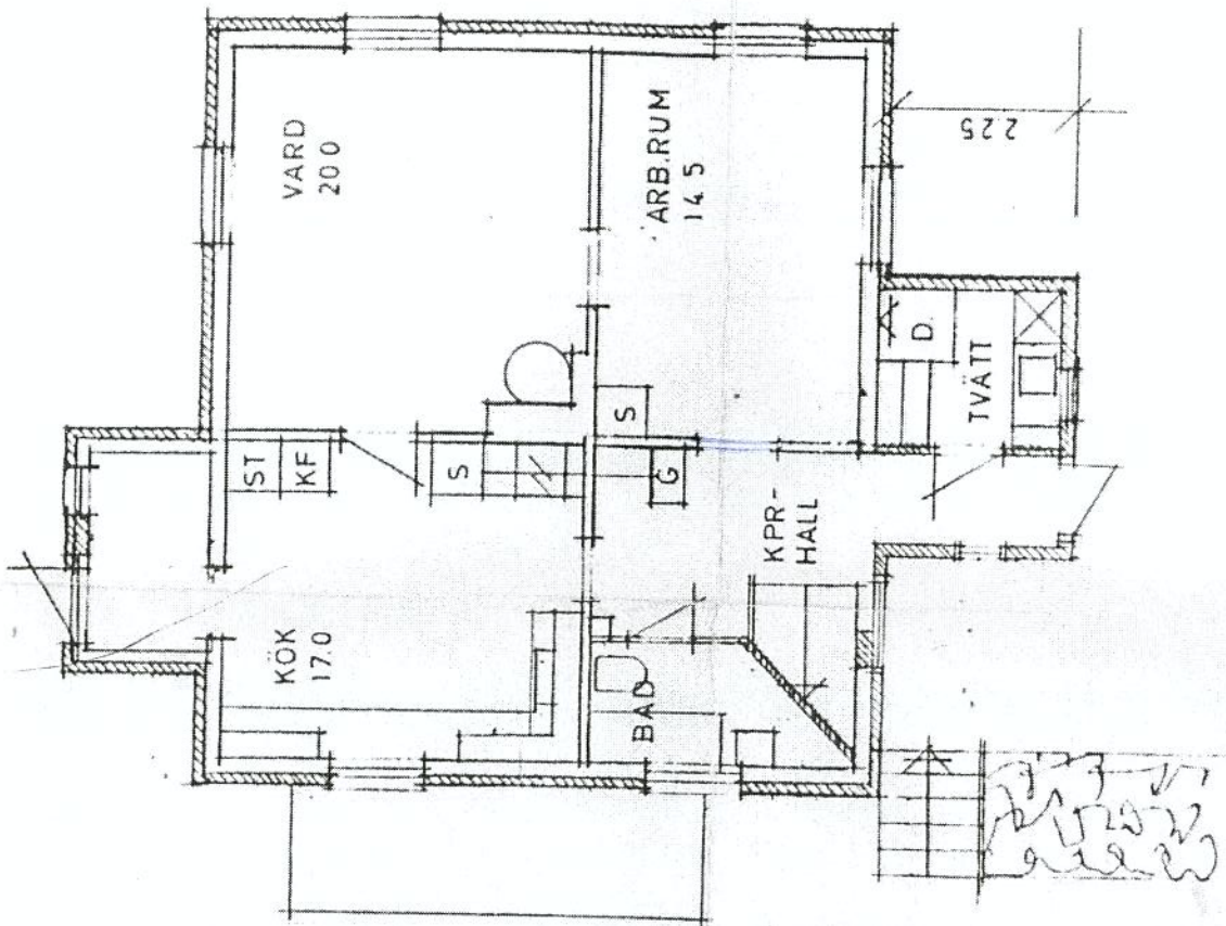
BOTTENPLAN
