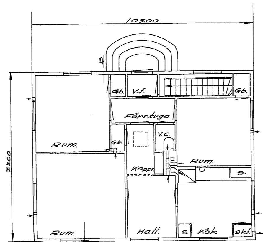
BOTTENPLAN
