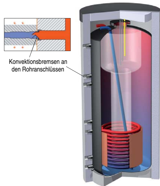
Wagner TERMO-Kombispeicher
