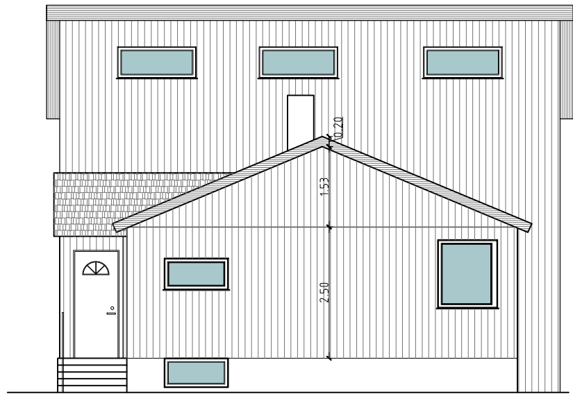
2 105 PROPOSED DRAWINGS - RIGHT ELEVATION SCALE 1:100 • A4
